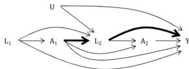
C. Condition on L_k \rightarrow over-control of intermediate pathways
