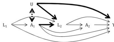
D. Condition on L_k \rightarrow collider-stratification bias
