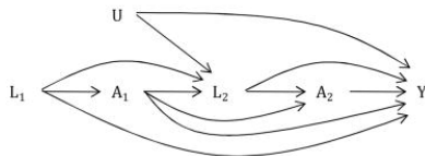
A. Hypothesized causal relationships
